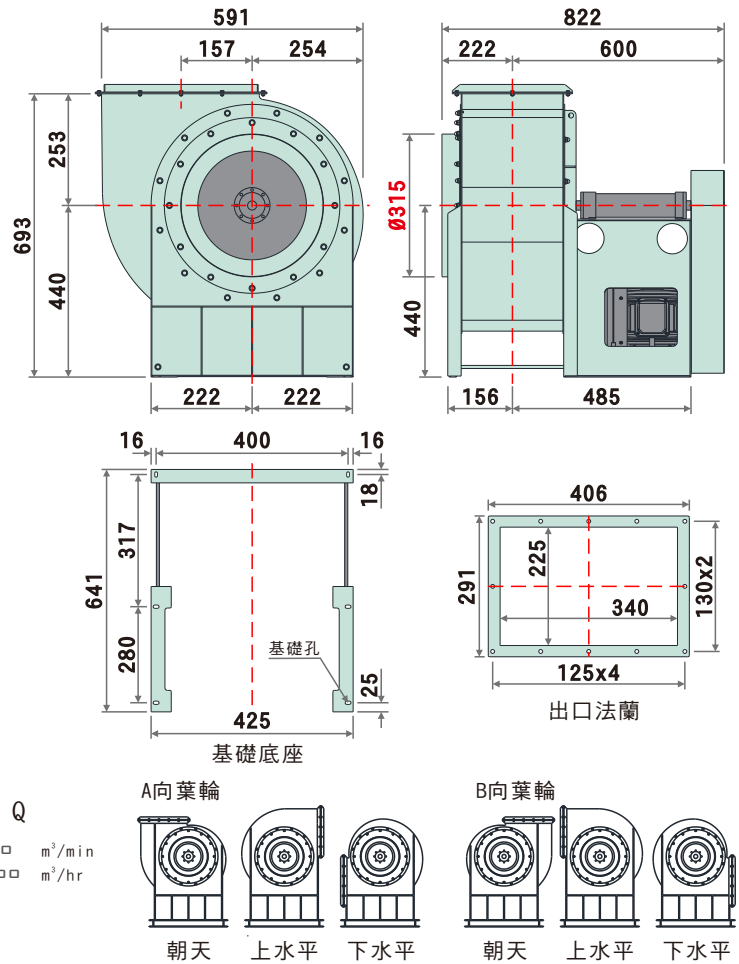
裝配方向視圖與尺寸 (DIMENSIONS)
